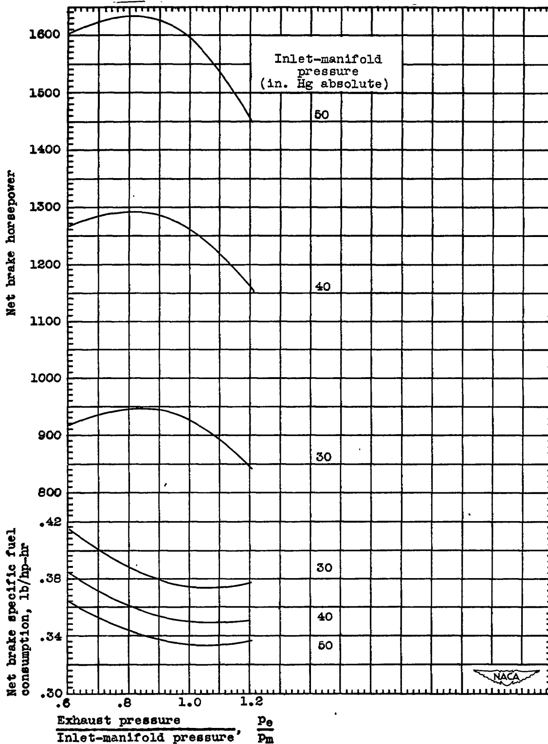
Figure 4. - Effect of p_e/p_m and inlet-manifold pressure on net brake horsepower and net brake specific fuel consumption. Engine speed, 2600 rpm; fuel-air ratio, 0.069; altitude, 30,000 feet.
