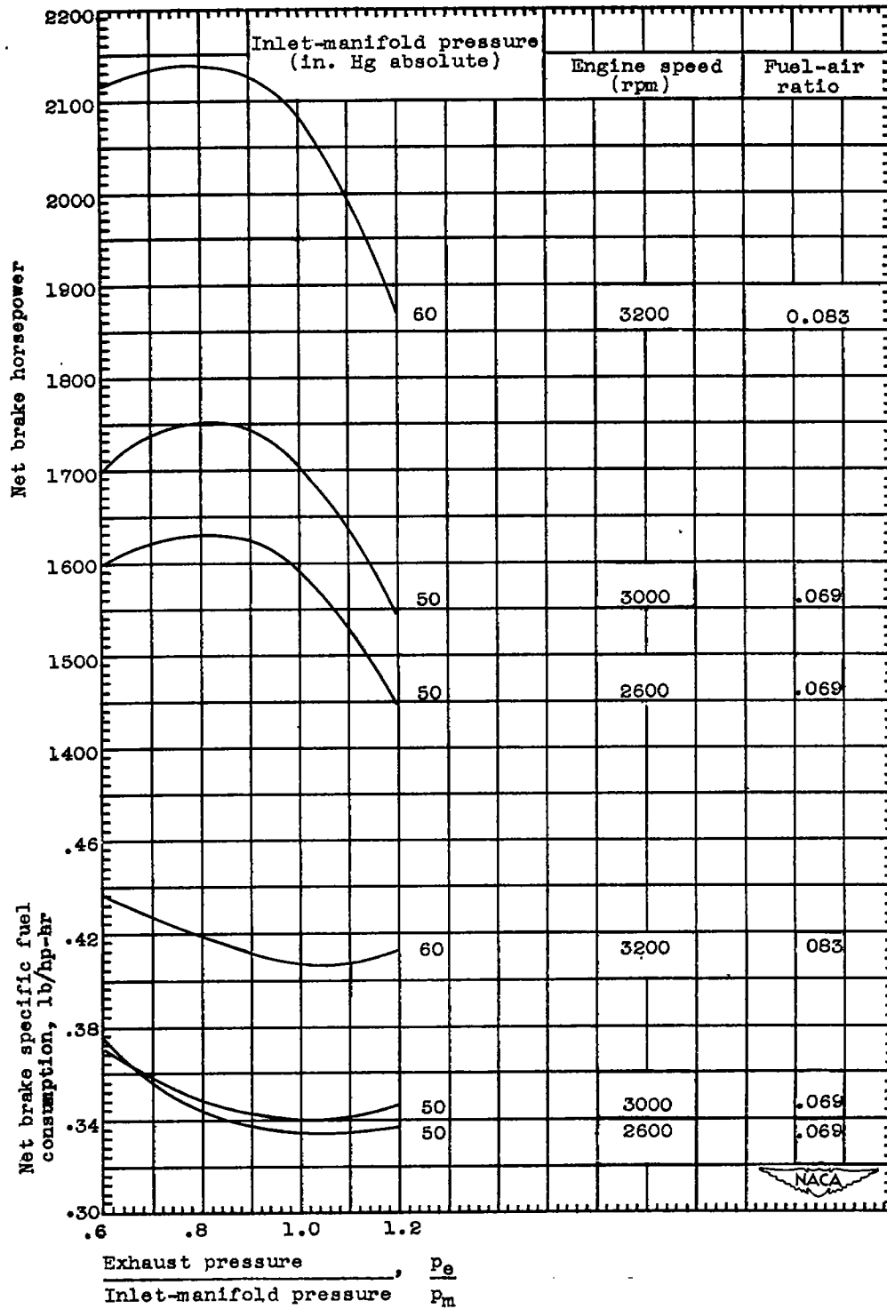
Figure 8. - Effect of p_e/p_m on high-power performance. Altitude, 30,000 feet.
