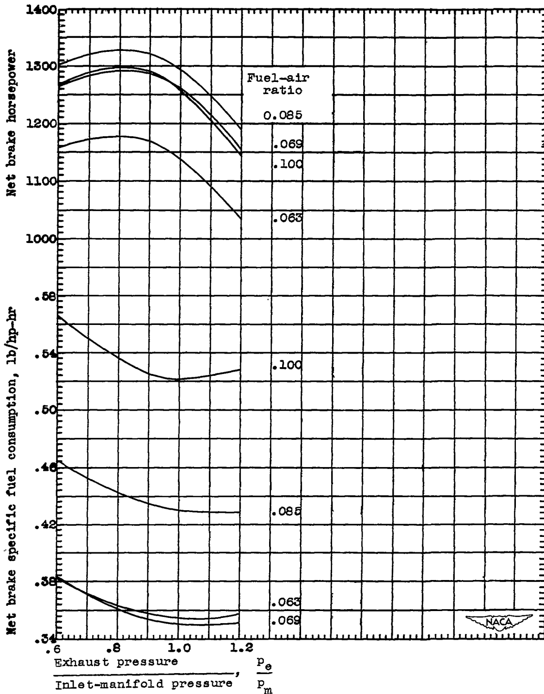
Figure 3. - Effect of p_e/p_m and fuel-air ratio on net brake horsepower and net brake specific fuel consumption. Engine speed, 2600 rpm; inlet-manifold pressure, 40 inches mercury absolute; altitude, 30,000 feet.
